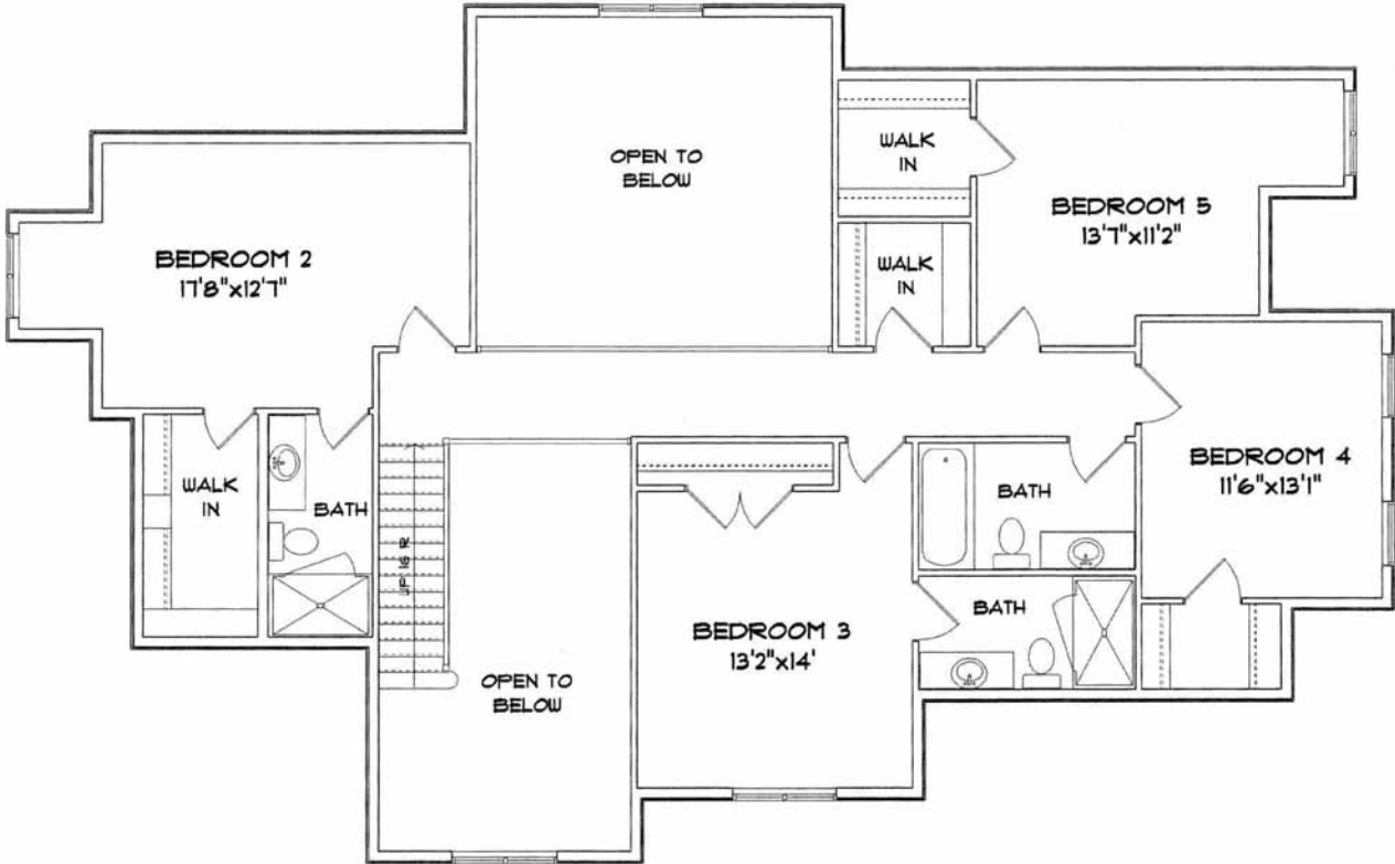
2ND FLOOR PLAN 1460.3 sq/ft
