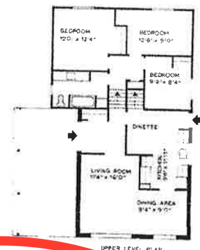
UPPER LEVEL PLAN
