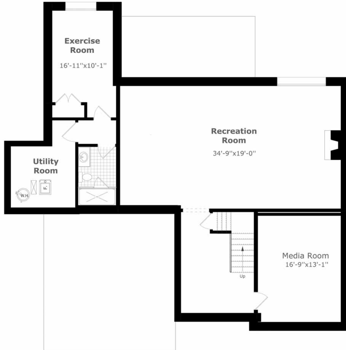
Basement Plan
