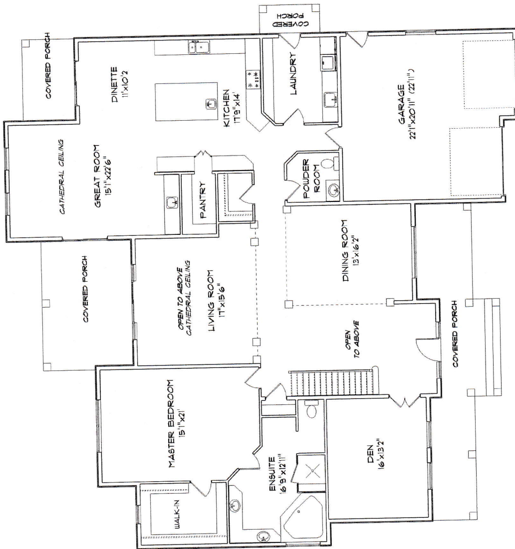
1ST FLOOR PLAN 2801 sq./ft. (260.23 sq.m.)
