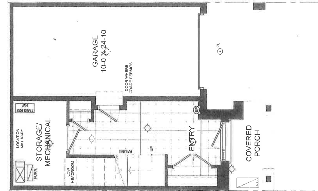
THE ALGROVE THB2B21-01 8M ELEVATION A GROUND FLOOR PLAN
