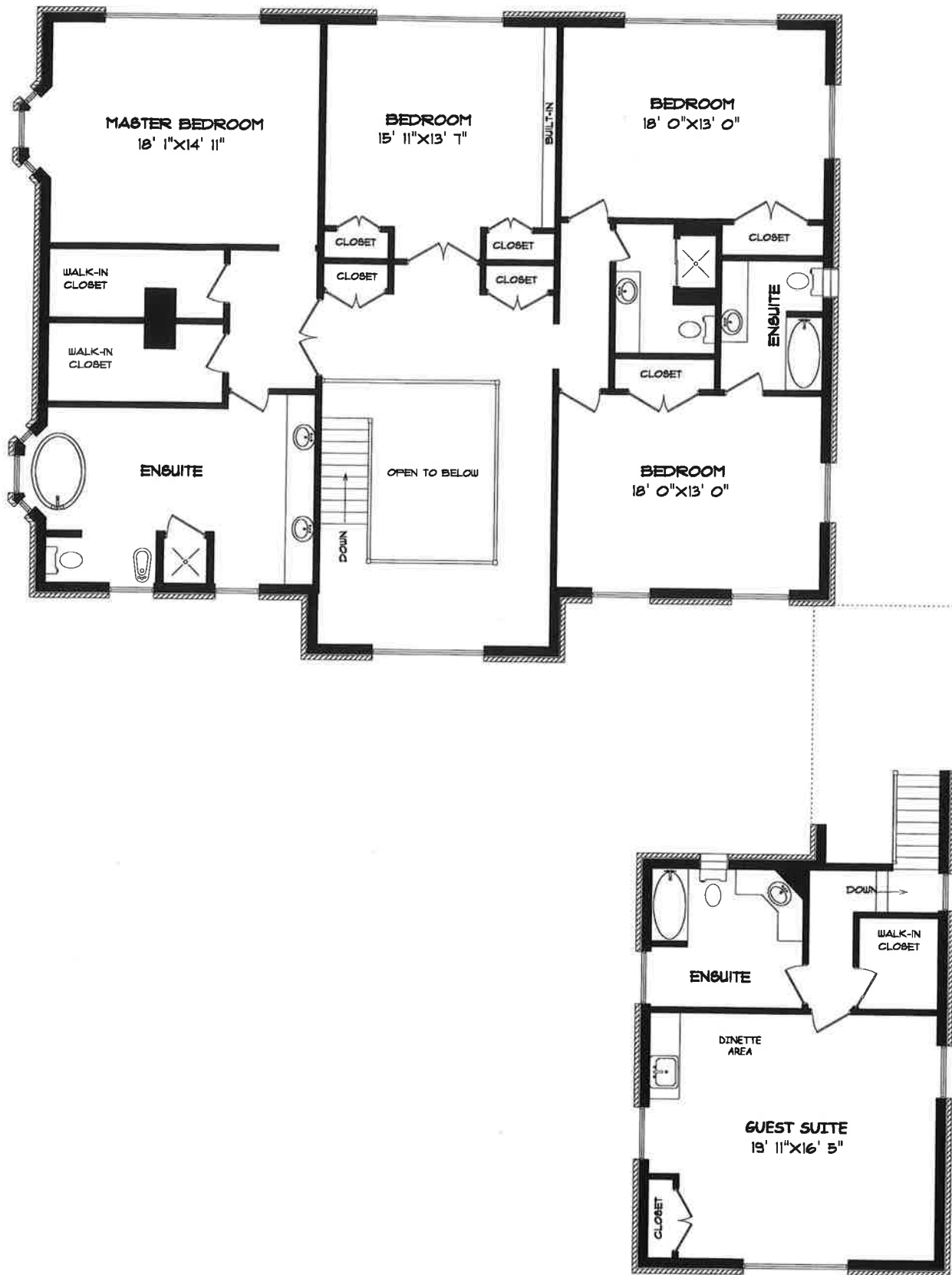
SECOND FLOOR 2782 SQUARE FEET
