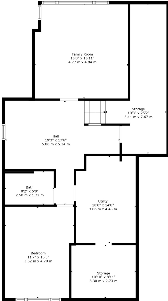
Floor 1
